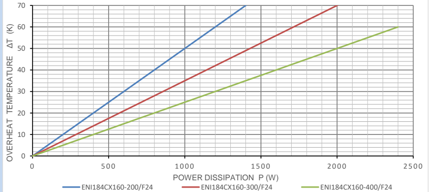
FORCED AIR-COOLING HEATSINKS THERMAL CHARACTERISTIC @ OUTGOING AIR-FLOW RATE 7.0 M/S
