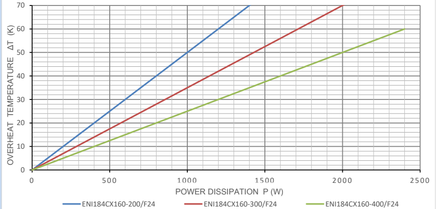
FORCED AIR-COOLING HEATSINKS THERMAL CHARACTERISTIC @ OUTGOING AIR-FLOW RATE 7.0 M/S
